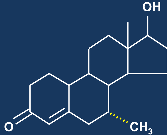
7 \alpha -Methyl-19-Nortestosterone (Synthetic high potency androgen)
